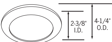
CTR311-(NK, P, ST) Frosted Flat Glass
