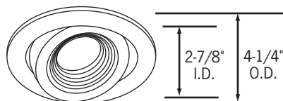
CTR307-(P, B, C, NK) Adjustable Pin Spot, Black Baffle
