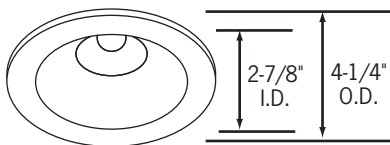
CTR302-P-(CLR, BLK, WHT) Adjustable Multiplier, White Trim Ring, Select Reflector Finish
