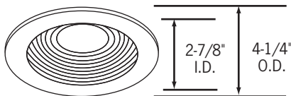
CTR301-P Adjustable Black Baffle
