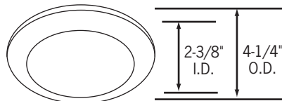
CTR313-P Convex Drop Lens Shower light trim. 3/4" Drop (ceiling to bottom of glass), double neoprene gasketed. cULus listed for wet location.
