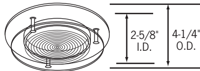
CTR315-(P, B, C) Glass Accent
