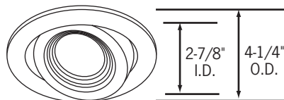
CTR306-P Surface Adjustable Black Baffle 40° Vertical adjustment, 359° horizontal rotation. 50mm Lens. Regressed black baffle reduces surface brightness. Flat, stainless mounting clips hold trim firmly to ceiling.
