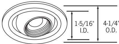
CTR308-P Adjustable Classic Eyeball, Black Baffle
