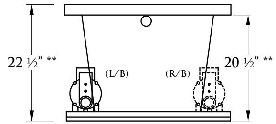
**Air option adds 1.5" to tub height. Components may extend beyond tub rim.
