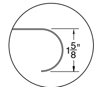
Bull Nose Edge Detail (On Front Only)
