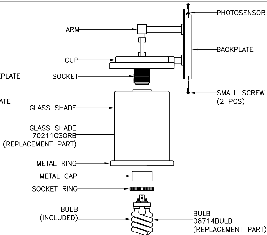
SIDE VIEW
