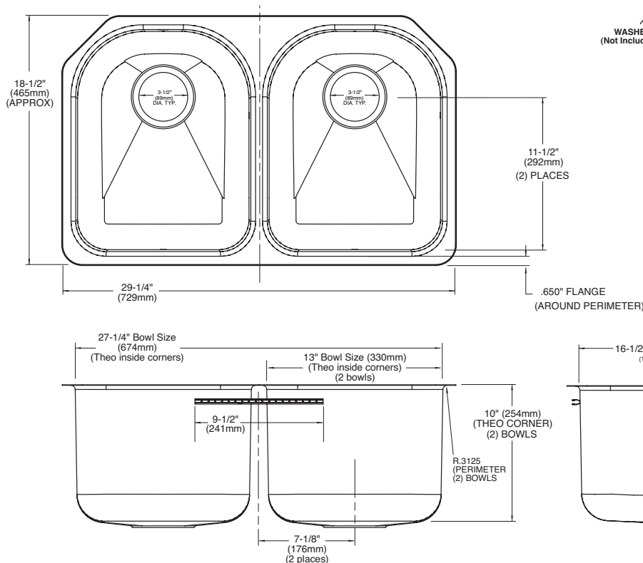
Installation Detail
