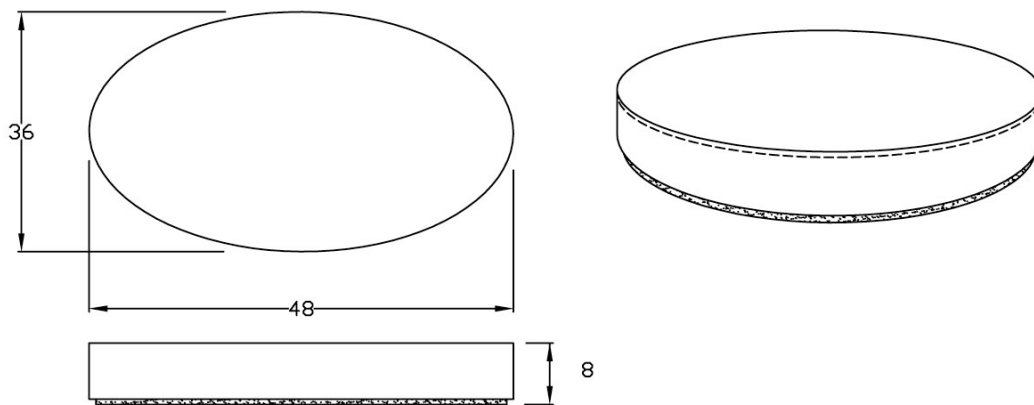
TECHNICAL RENDERINGS WITH DIMENSIONS (IN INCHES)
