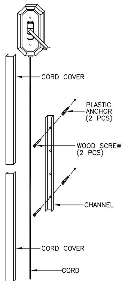
CORD COVER ASSEMBLY
