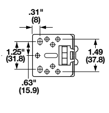
Rear Metal Bracket
