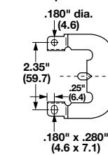
Front Clip-on Bracket
