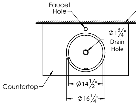
TOP VIEW DROP-IN APPLICATION
