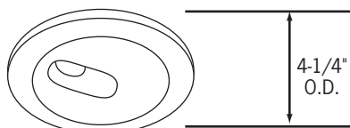
CTR303NMH-P Slotted Wall Wash 1-3/8" x 2-1/2" Oblong Slot 50° Swing adjustment, external 358° rotation. Slot aperture permits maximum beam area adjustment for either wall wash or concealed accent lighting effects. Black interior surface, (1) 45mm lens option.
