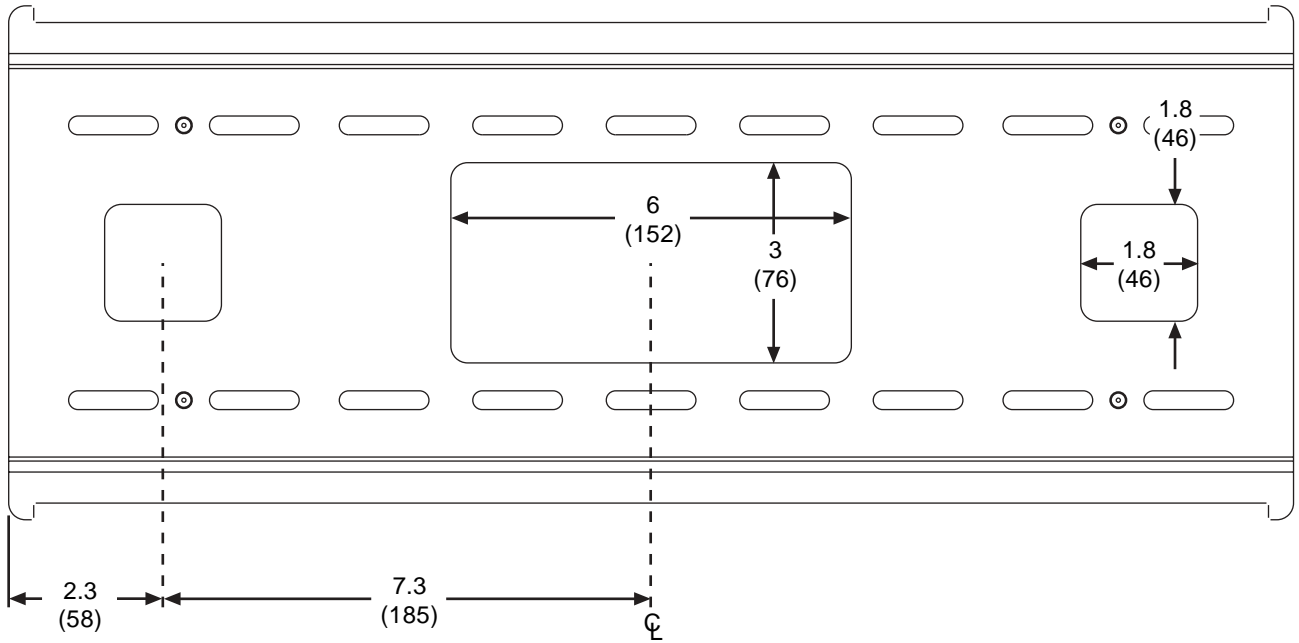
Wall Plate Detail
