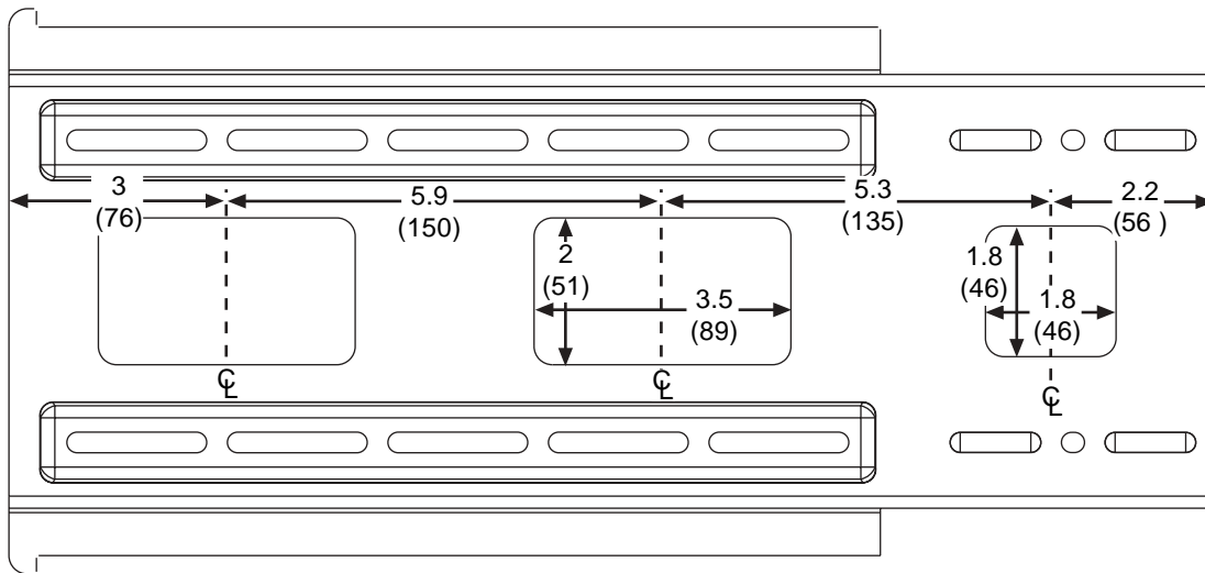
Wing Bracket Detail
